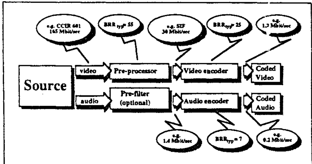
Figure 3 Typical audio and video encoding environment
