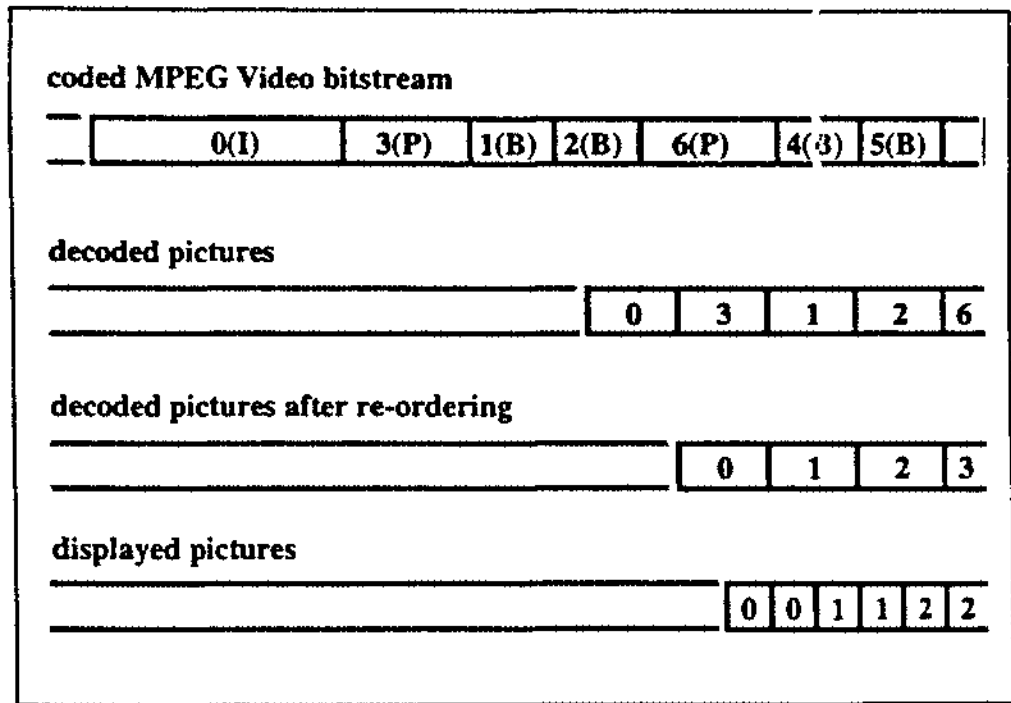
Figure 6 MPEG Video decoding
