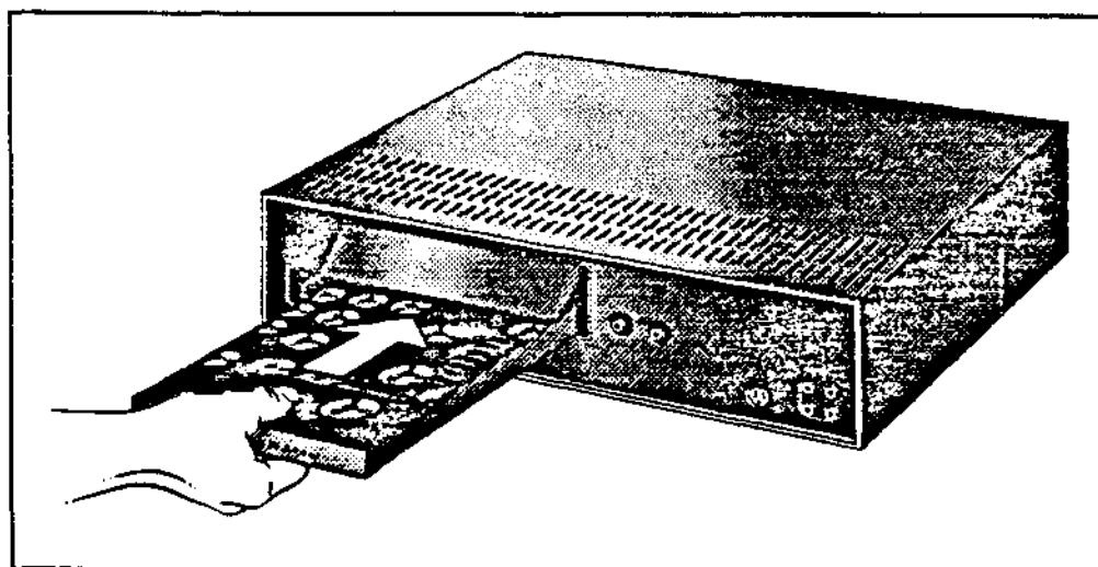
Figure 1 Installing a Full Motion cartridge in a Base Case CD-I player prepared for Full Motion.
