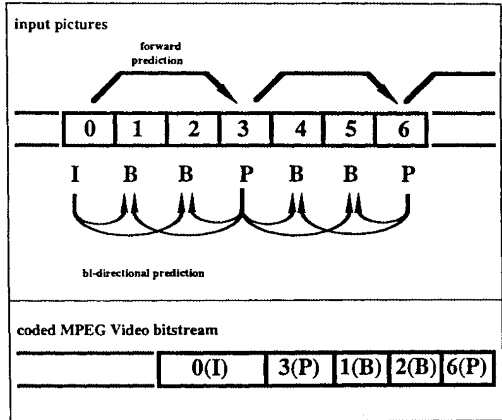
Figure 4 MPEG Video encoding
