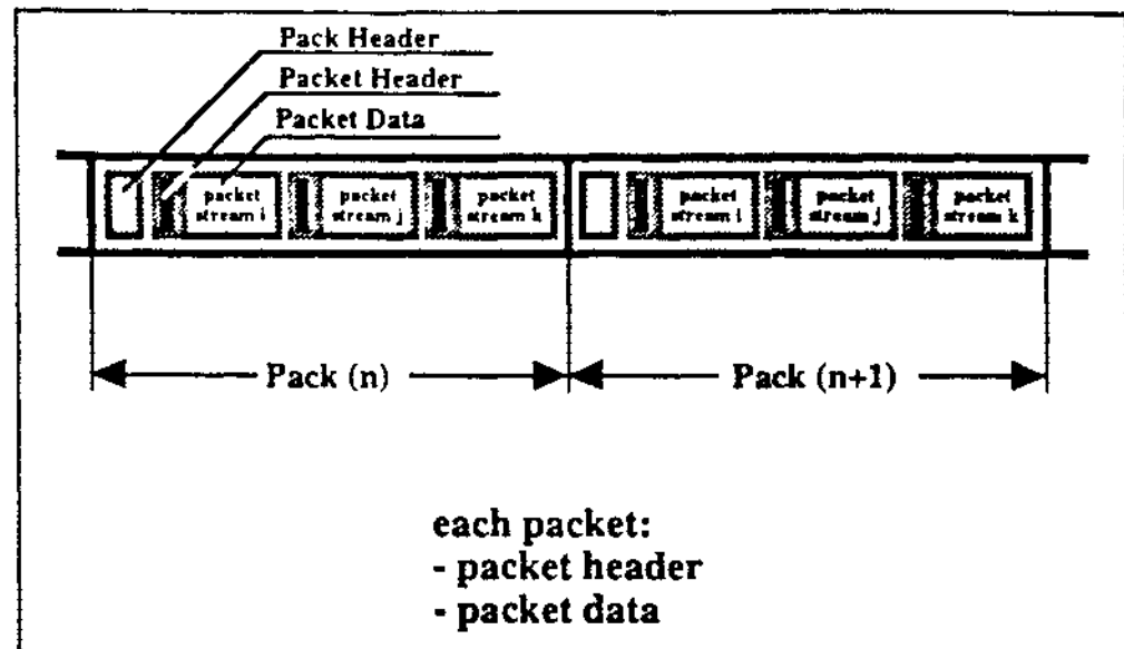
Figure 13 Example of MPEG multiplex structure with three streams (i, j and k).
