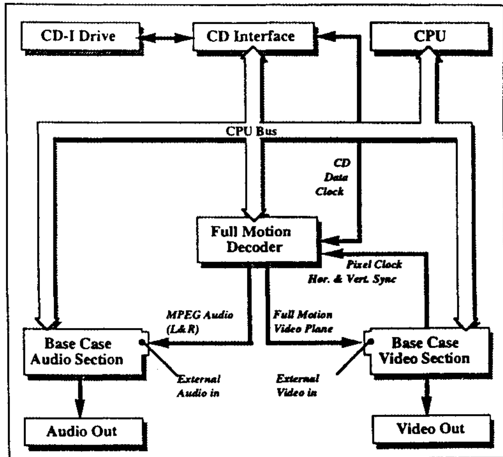
Figure 16 Full Motion decoder in a CD-I player
