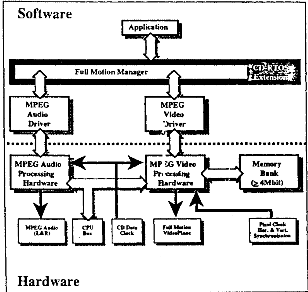
Figure 17 Structure of Motion decoder
