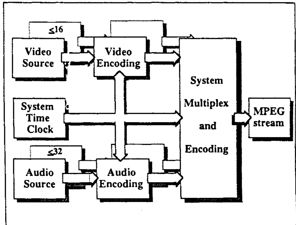
Figure 12 General MPEG encoding system
