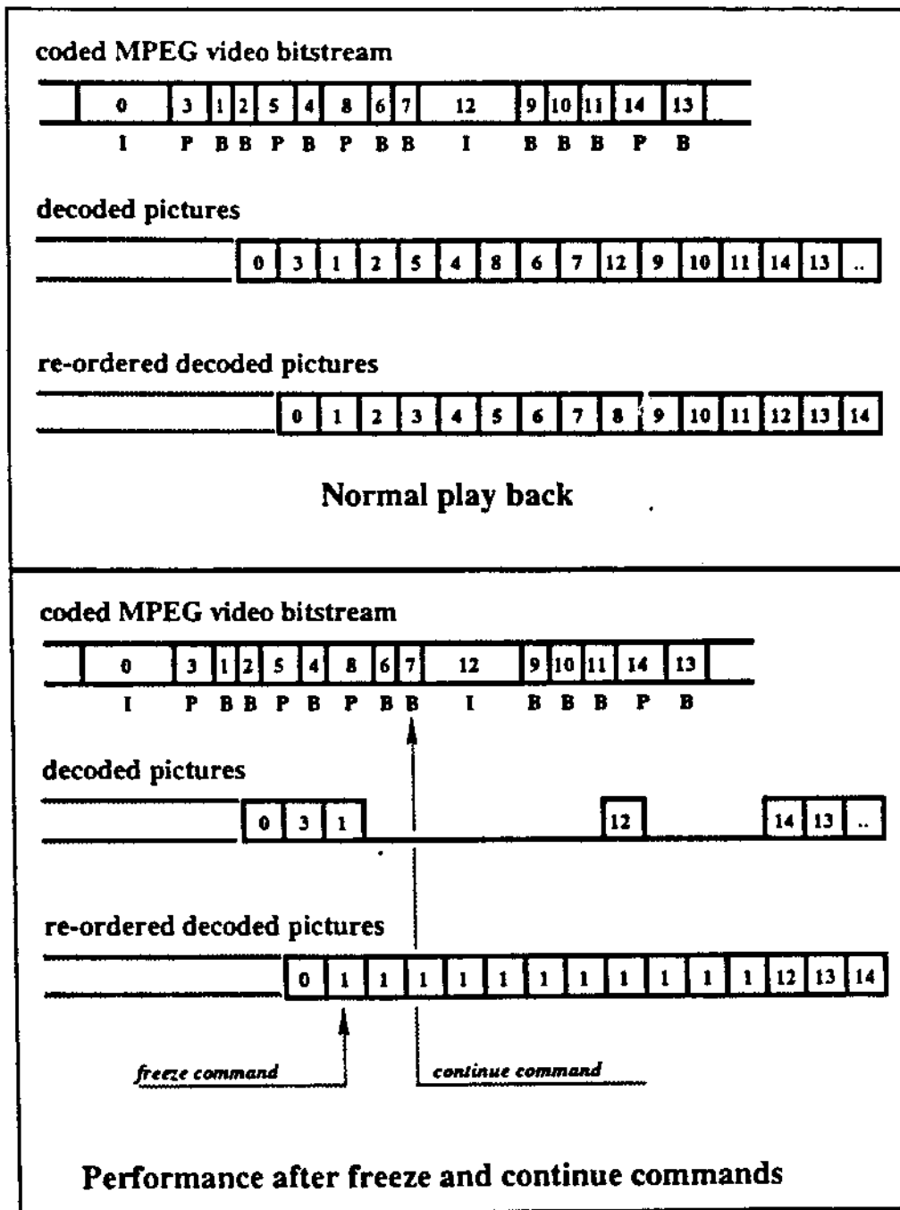
Figure 8 Normal play back and performance after freeze and continue commands; in this example the freeze command is issued during display of picture no 1, while the continue command is issued prior to encountering picture no 12 in the MPEG video bitstream
