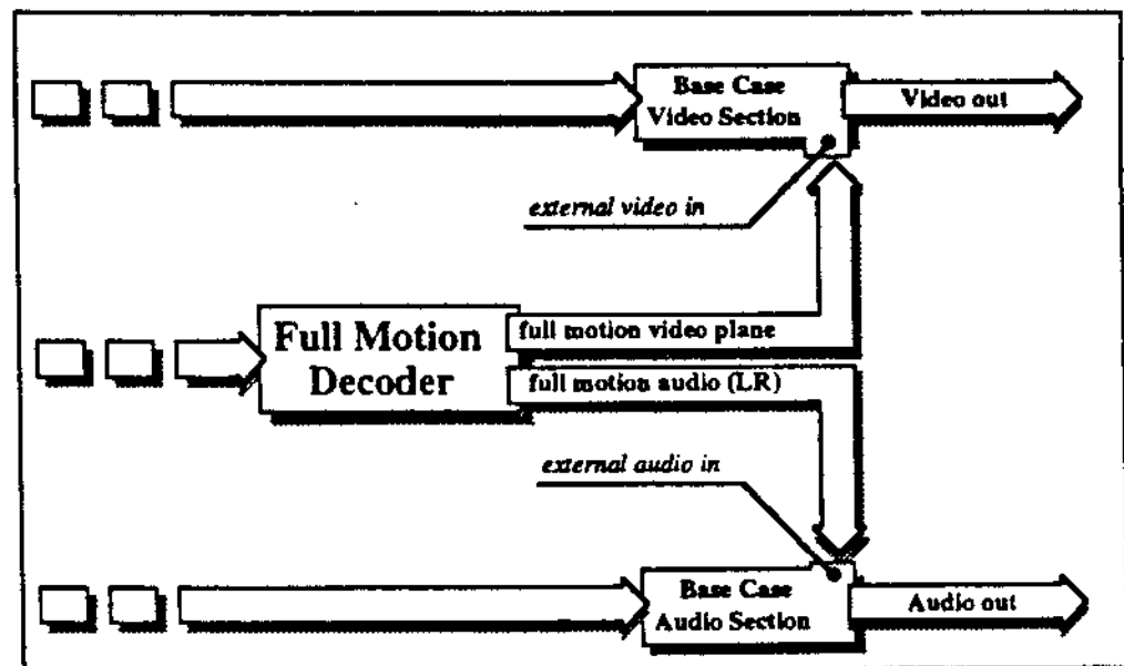
Figure 5 Mixing of audio and video from Full Motion decoder with Base Case audio and video
