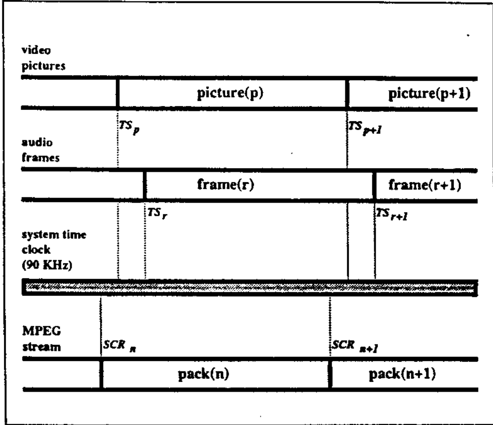
Figure 14 Synchronization between audio and video in MPEG, using the 90 kHz System Time Clock.
